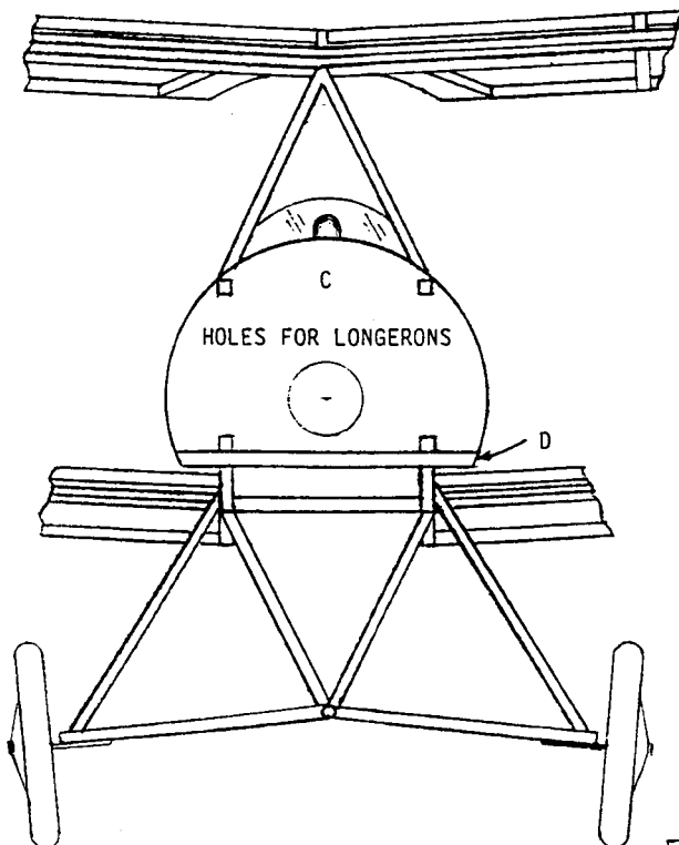
FULL SIZE FRONT L.G. STRUTS MAKE OVER DI AN
